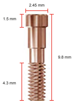
Laborschraube Laboratory Screw
